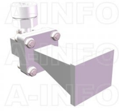
LB-62-10-C-7SPO Standard Gain Horn Antenna 12.4-18GHz 10dB Gain 7mm
